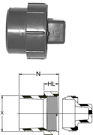
Cleanout Adapter with Plug (Spg x FT)
