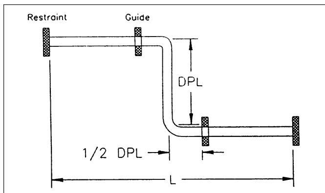
Figure C: Expansion Offset
