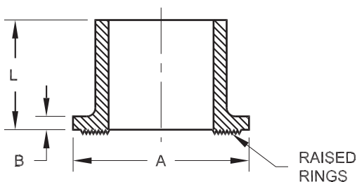
Factory Mutual IPS Flange Adapter
